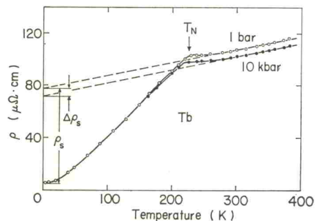
Fig. 2. Electrical resistivity as a function of temperature.
